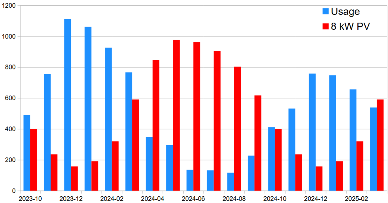
Figure 4: Projected usage and production with an 8 kW Solar PV system
